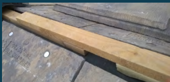
Gaps can be created by using two battens with spaces. In this photo, the ridge roll was omitted (they often contain BRM) and the battens placed directly onto Type 1F 1F bitumen felt. Screws go through the clip/bracket and into the ridge board.
